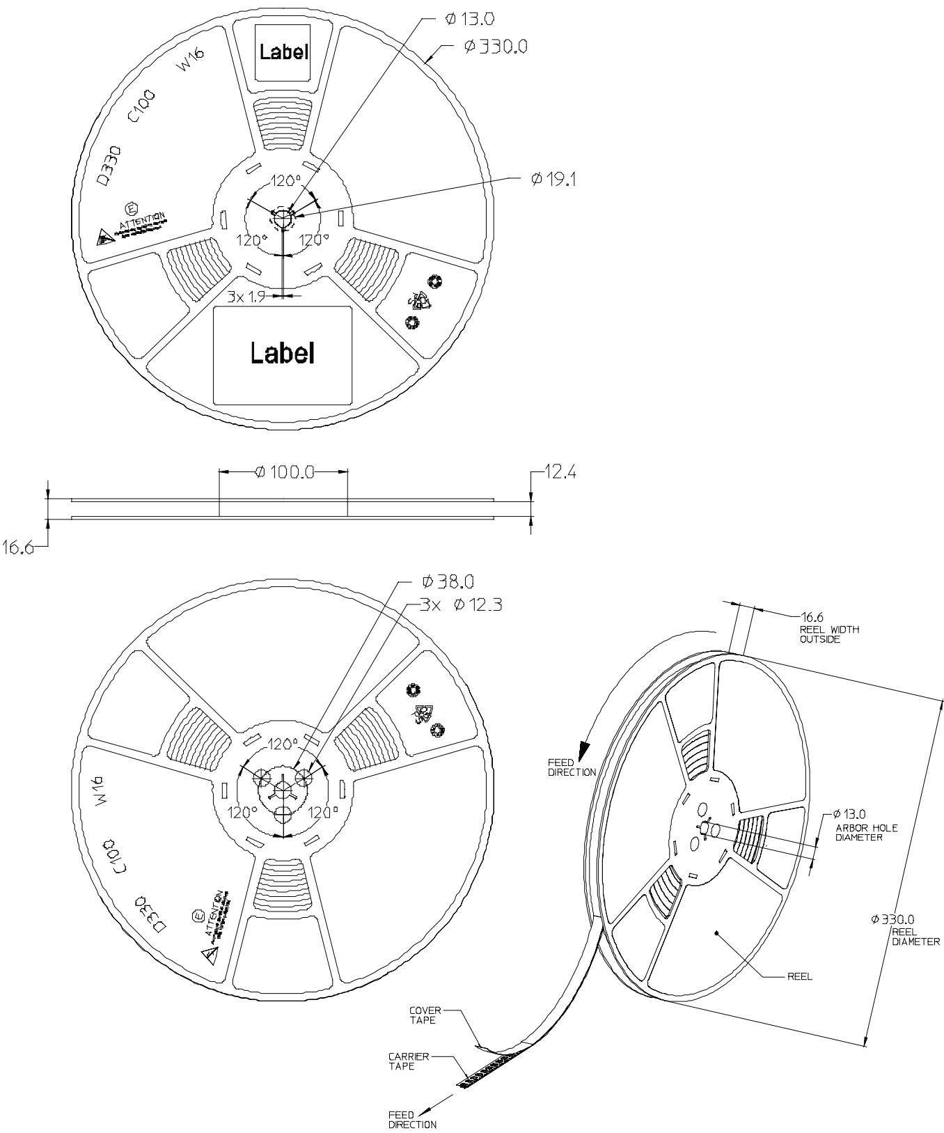
Figure 14. Emitter reel packaging
