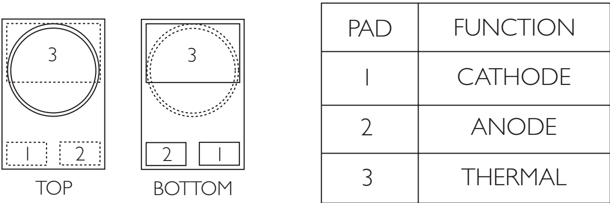
Figure 2. Pad configuration.
