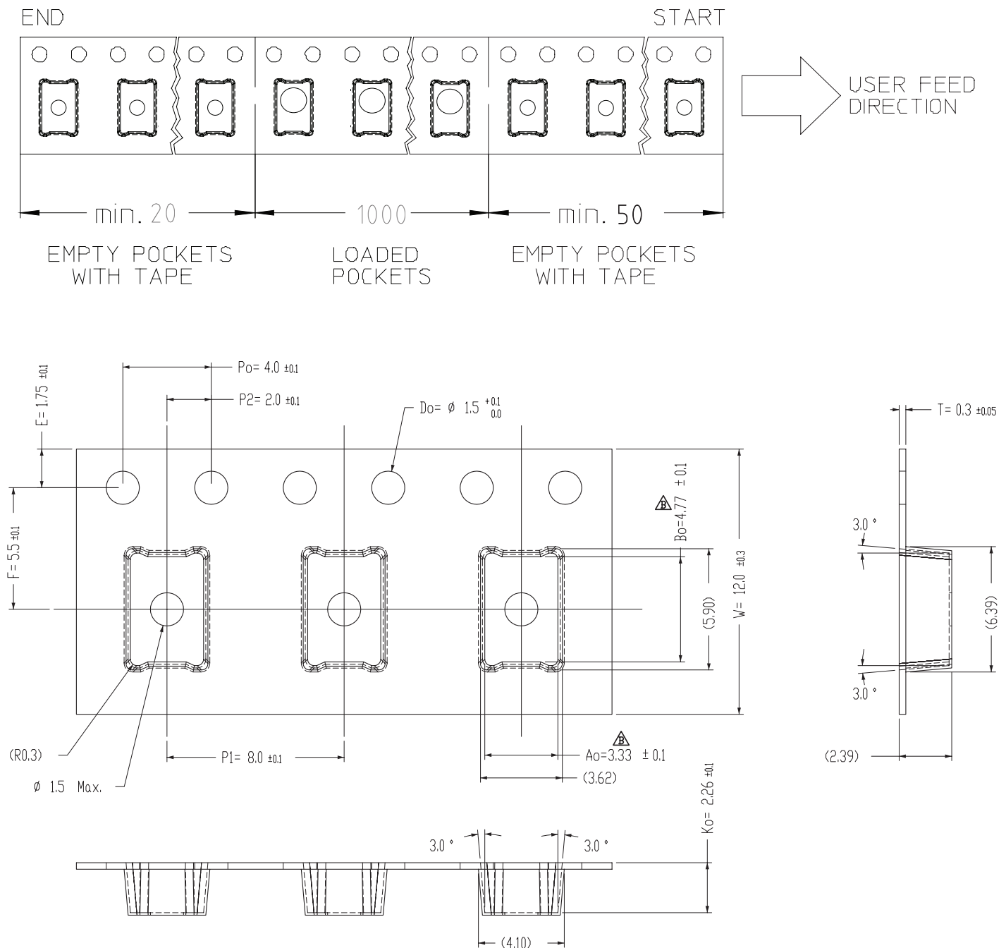
Figure 13. Emitter pocket tape packaging
